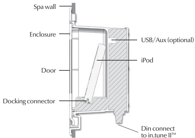
Side view in.p3-110™
